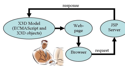
Figure 3: Client-Server Interaction.
