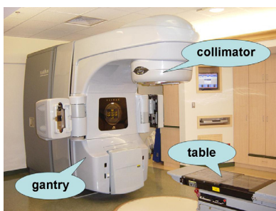
Figure 1: Linear accelerator with on-board imaging.
