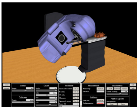
Figure 4: 3DRTT with HTML/JavaScript-based GUI
