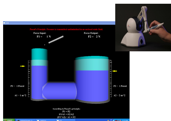
Figure 8: HaptEK16 screenshot and corresponding Phantom® Omni™ device from Sensable Technologies
